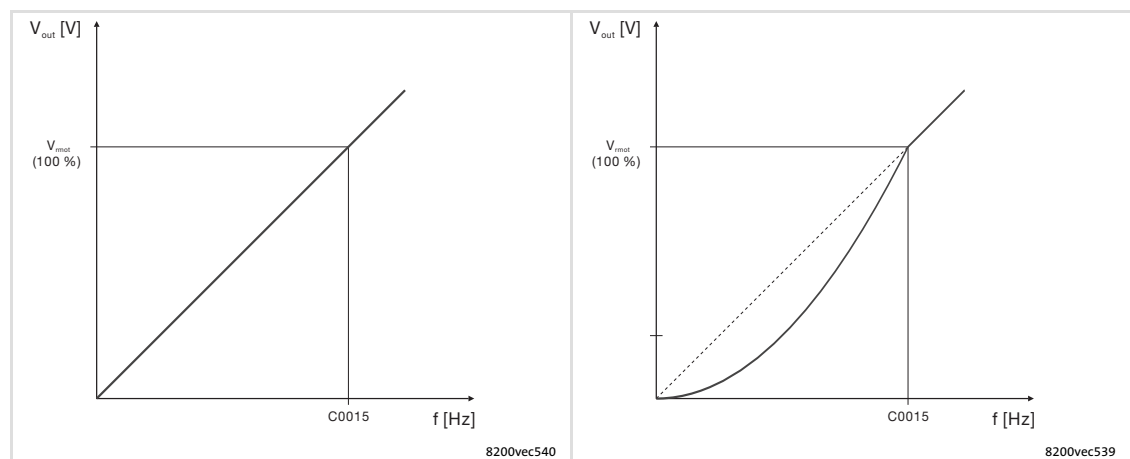
Fig. 10-2 Linear and square-law V/f characteristic
