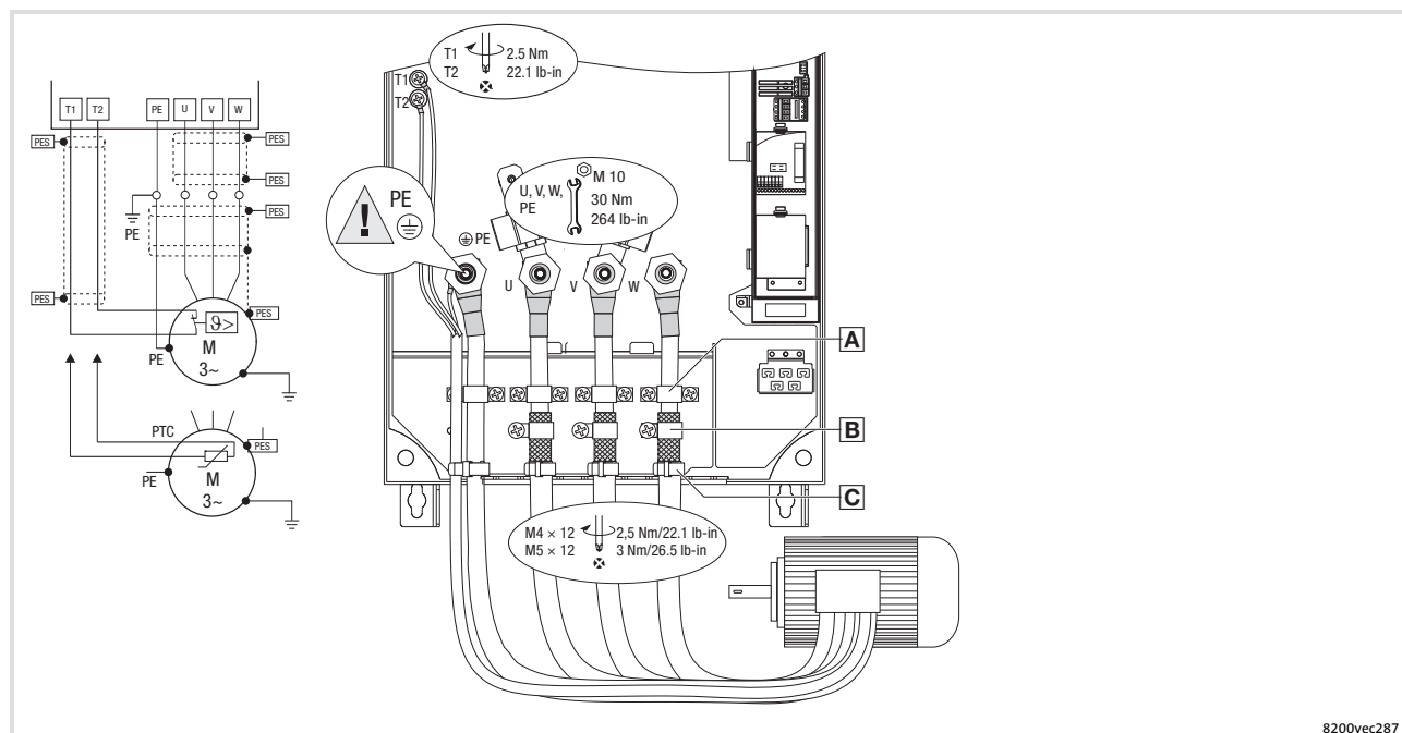
Fig. 6-27 Motor connection 75 ... 90 kW
