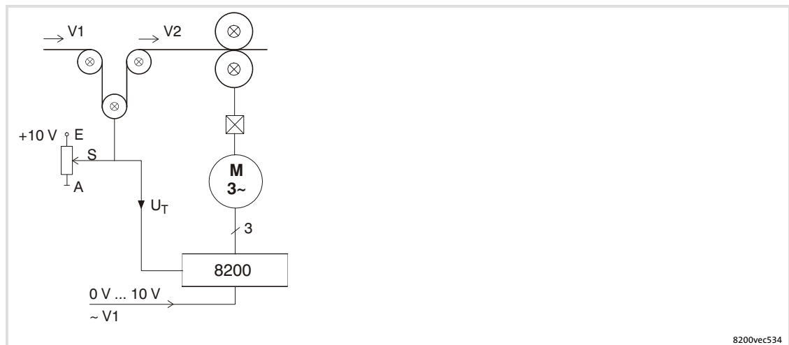
Fig. 10-13 Example: Dancer control with adding influence of the process controller
